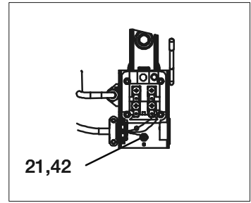
PRESSURE SWITCH WIRING
